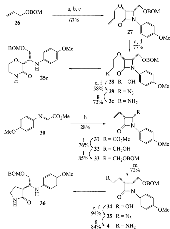
Scheme 5. a) \text{O}_3 , \text{CH}_2\text{Cl}_2/\text{MeOH} , then \text{Me}_2\text{S} ; b) p -anisidine, mol. sieves; c) allyloxyacetyl chloride, \text{CH}_2\text{Cl}_2 , \text{Et}_3\text{N} , -20\text{ }^\circ\text{C} to room temp.; d) \text{BH}_3\cdot\text{THF} ; e) \text{MsCl} , \text{Et}_3\text{N} , \text{CH}_2\text{Cl}_2 , -30\text{ }^\circ\text{C} ; f) \text{NaN}_3 , \text{DMF} , 50\text{--}60\text{ }^\circ\text{C} ; g) \text{Ph}_3\text{P} , \text{H}_2\text{O}/\text{THF} , room temp.; h) crotonyl chloride, \text{Et}_3\text{N} , \text{CH}_2\text{Cl}_2 , reflux; i) \text{Ca}(\text{BH}_4)_2 , \text{THF}/\text{EtOH} ; l) \text{BOMCl} , \text{Et}_3\text{N} , \text{CH}_2\text{Cl}_2 , reflux; m) 9-BBN, \text{THF} , room temp.; then \text{KHCO}_3 , \text{H}_2\text{O}_2
