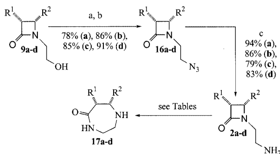
Scheme 3. a) \text{MsCl} , \text{Et}_3\text{N} , \text{CH}_2\text{Cl}_2 , -30\text{ }^\circ\text{C} ; b) \text{NaN}_3 , \text{DMF} , 50\text{--}60\text{ }^\circ\text{C} ; c) \text{Ph}_3\text{P} , \text{H}_2\text{O}/\text{THF} , room temp.
